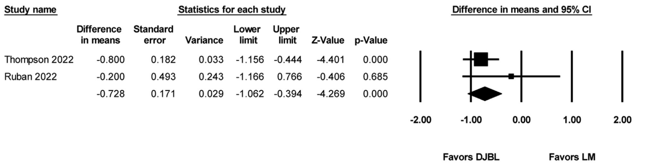
Supplementary Figure 4. Forest plot of the mean difference, representing the difference in pooled change in HbA1c of the DJBL group minus that of the control group, at 12 months (BMI 30-39.9 kg/m 2 ). Data derived from randomized controlled trials of DJBL. I^2 = 23.4 ; P = .25 . BMI , Body mass index; DJBL , duodenal-jejunal bypass liner; CI , confidence interval; LM , lifestyle modification.
